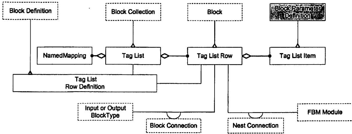
Figure 106 - Tag List Object Model
